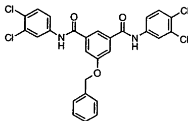
Compound # 43
